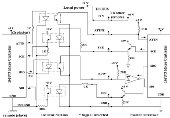
Fig. 5 Edbus Circuit Diagram
