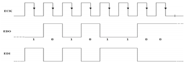
Fig. 6 Edbus Waveform
