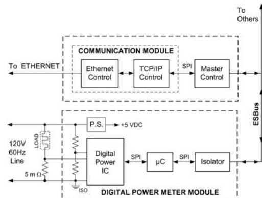
Fig. 4 Block Diagram of the Digital Power Meter with Ebus and Internet Interface
